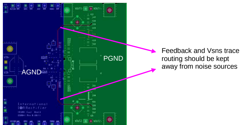
Figure 42c: IRDC3891 Demo board Layout Considerations – Mid Layer 1
