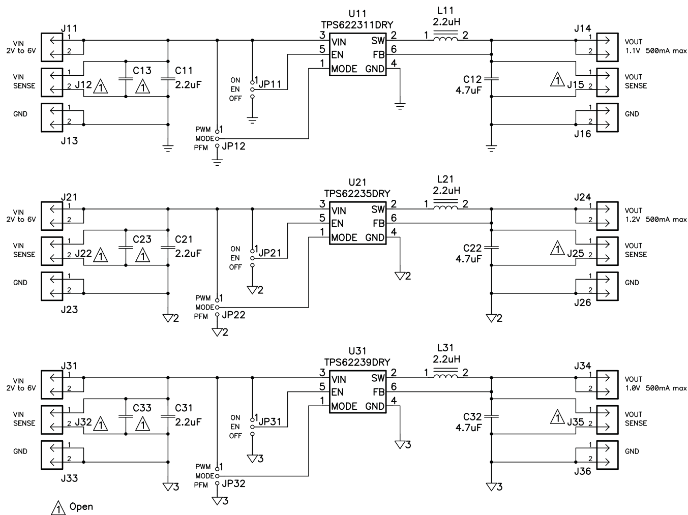
Figure 4. TPS62239EVM-574 Schematic
