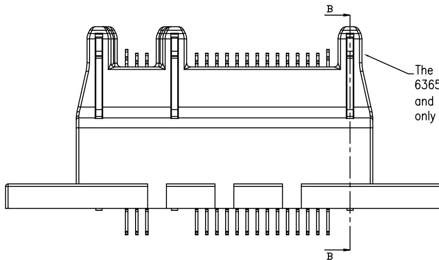
COUPE B-B (only for 63657-003LF)
