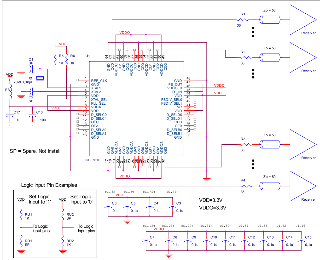
FIGURE 3. ICS8761I CLOCK GENERATOR SCHEMATIC EXAMPLE
