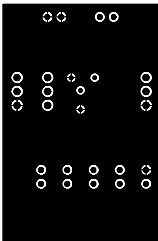
Figure 6. LP5524 Evaluation Board Layer 3.
