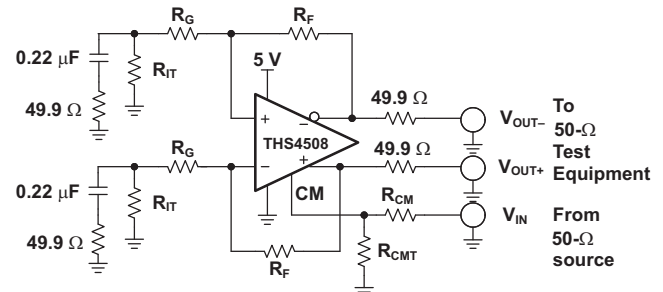
Figure 47. CM Input Test Circuit
