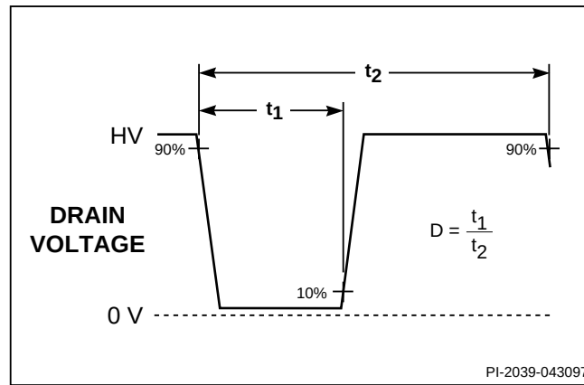
Figure 49. Duty Cycle Measurement.
