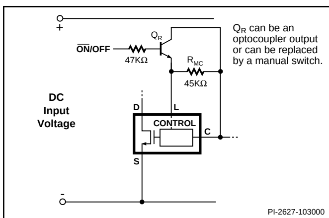
Figure 25. Active-off Remote ON/OFF. Maximum Duty Cycle will be reduced.
