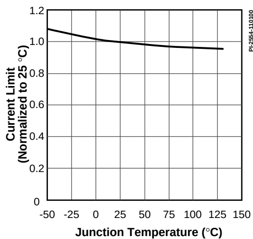
Figure 58. External Current Limit vs. Temperature with R_{IL} = 12k\Omega .
