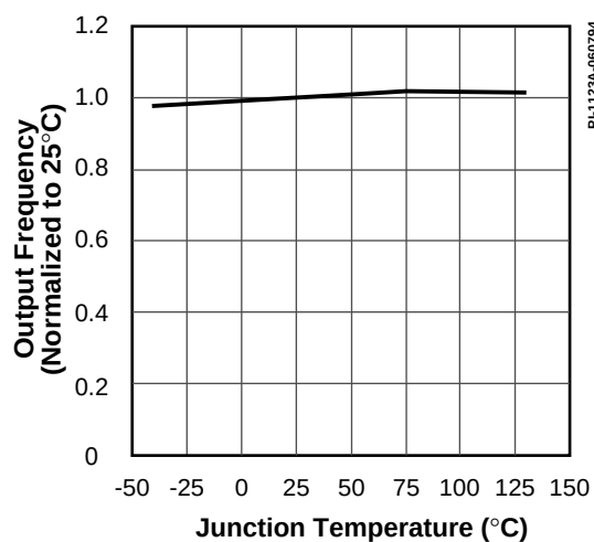
Figure 56. Frequency vs. Temperature.
