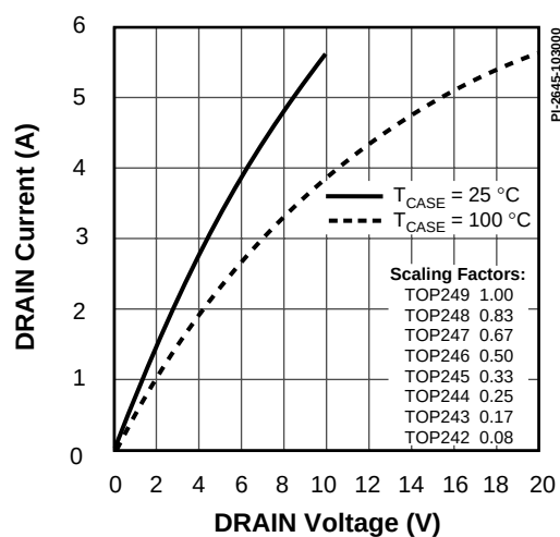
Figure 65. Output Characteristics.
