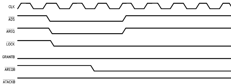
FIGURE 35. LOCK Function
