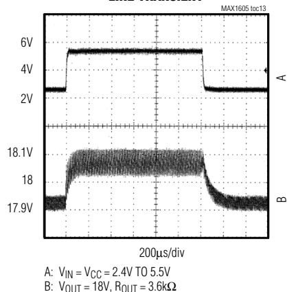
LINE TRANSIENT
