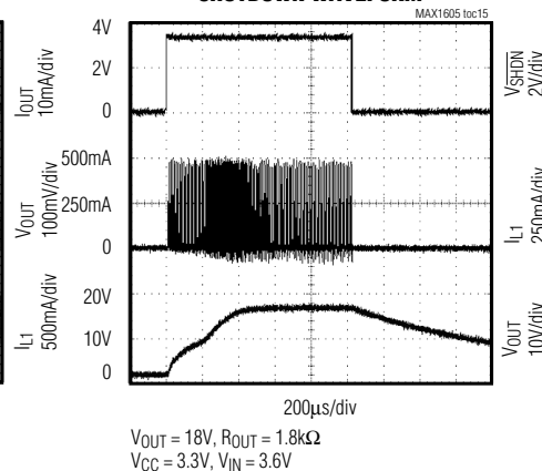
SHUTDOWN WAVEFORM
