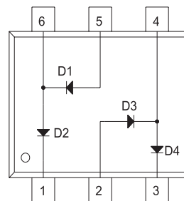
CMLD6263S Marking Code: 63S
