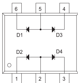
CMLD6263A Marking Code: 63A
