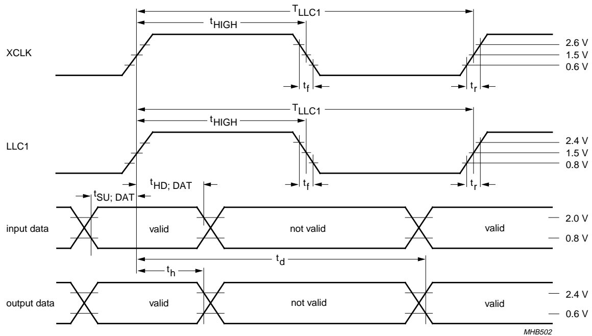
Fig.11 Clock data timing.
