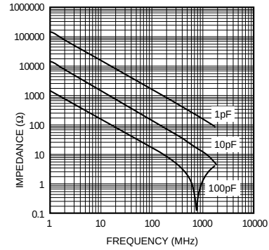
Fig.2 Impedance-frequency characteristics
