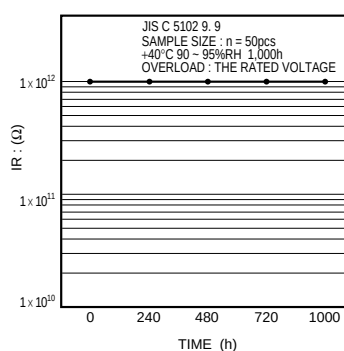
Fig.27 Insulation resistance
