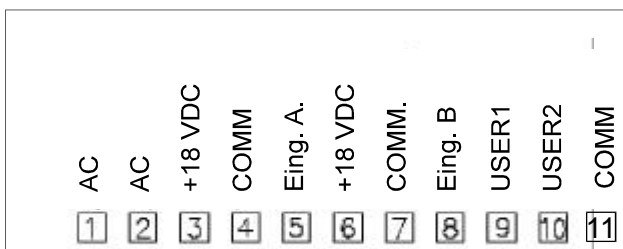
Anschlüsse PAXDP000
