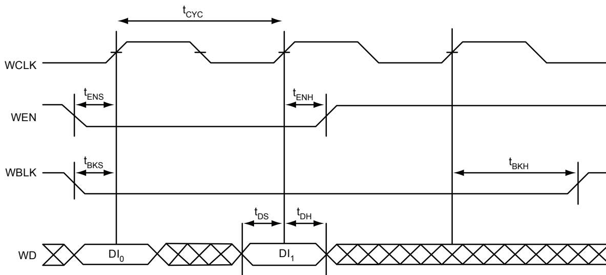
Figure 2-33 • FIFO Write
