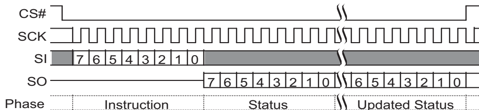
Figure 52. Read Status Register-2 (RDSR2 07h) Command Sequence
