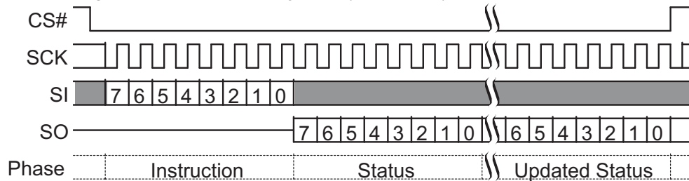
Figure 51. Read Status Register-1 (RDSR1 05h) Command Sequence
