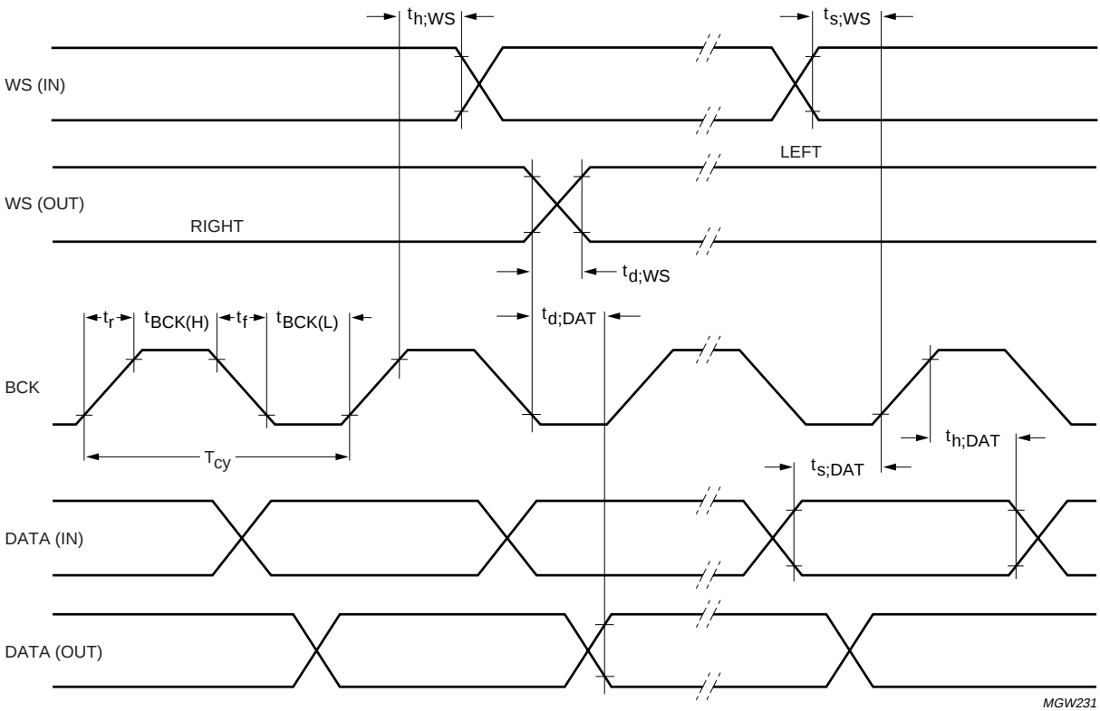
Fig.29 I²S-bus timing diagram for digital audio inputs/outputs.
