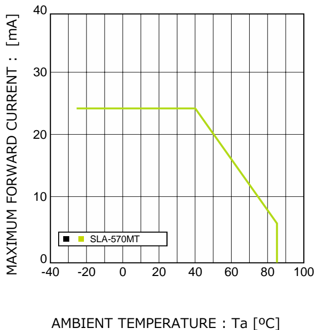
Fig.4 Derating
