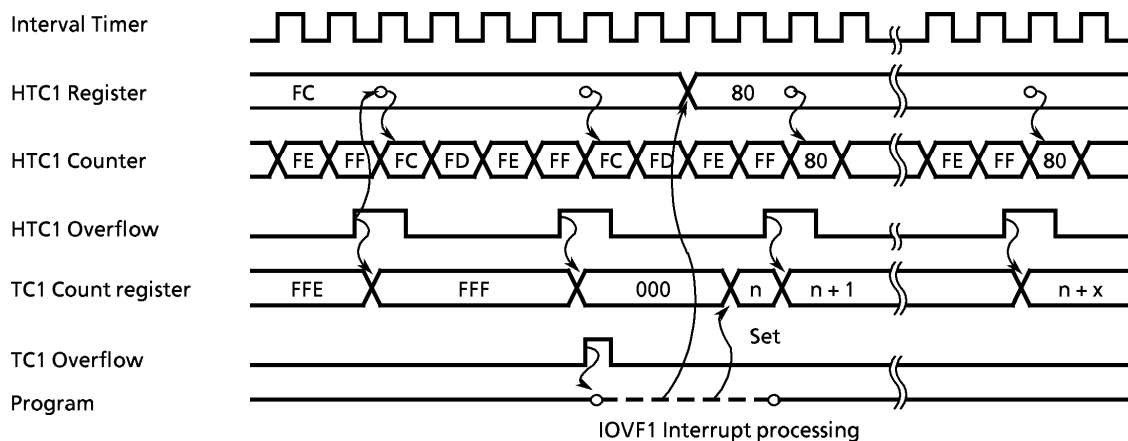
Figure 2-5. Timer mode
