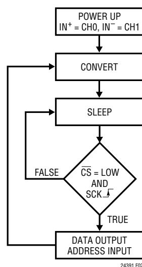
Figure 2. LTC2439-1 State Transition Diagram
