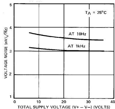
VOLTAGE NOISE DENSITY vs SUPPLY VOLTAGE
