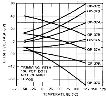
OFFSET VOLTAGE DRIFT OF EIGHT REPRESENTATIVE UNITS vs TEMPERATURE
