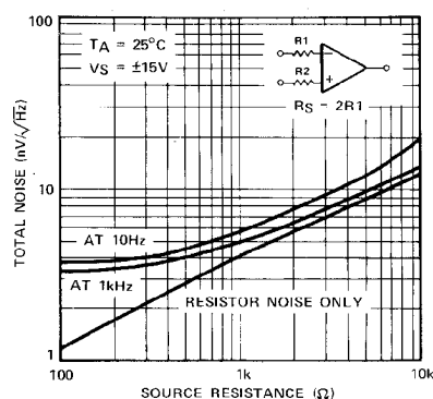
TOTAL NOISE vs SOURCE RESISTANCE
