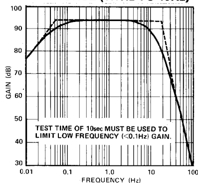
NOISE-TESTER FREQUENCY RESPONSE (0.1Hz TO 10Hz)
