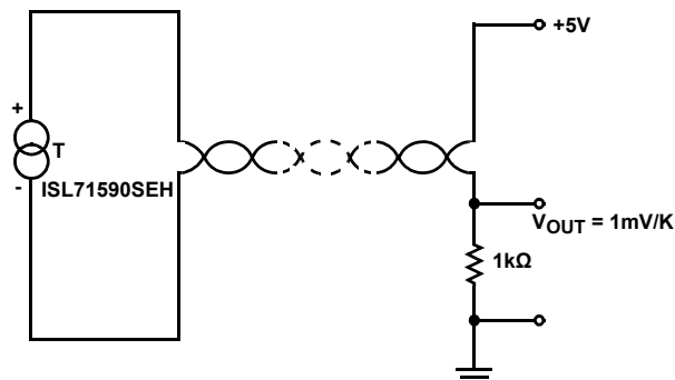
FIGURE 28. TYPICAL APPLICATION
