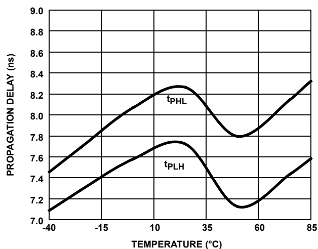
FIGURE 12. DRIVER DIFFERENTIAL PROPAGATION DELAY vs TEMPERATURE
