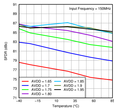
Figure 7-41. SFDR vs Temperature and AVDD Supply
