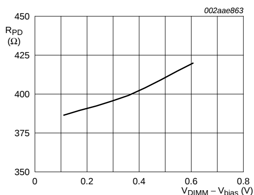
Fig 6. Pull-down resistance versus voltage
