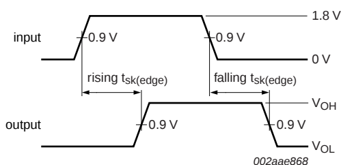
Fig 11. Rising and falling edge skew
