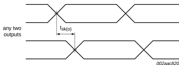
Fig 12. Skew between any two outputs
