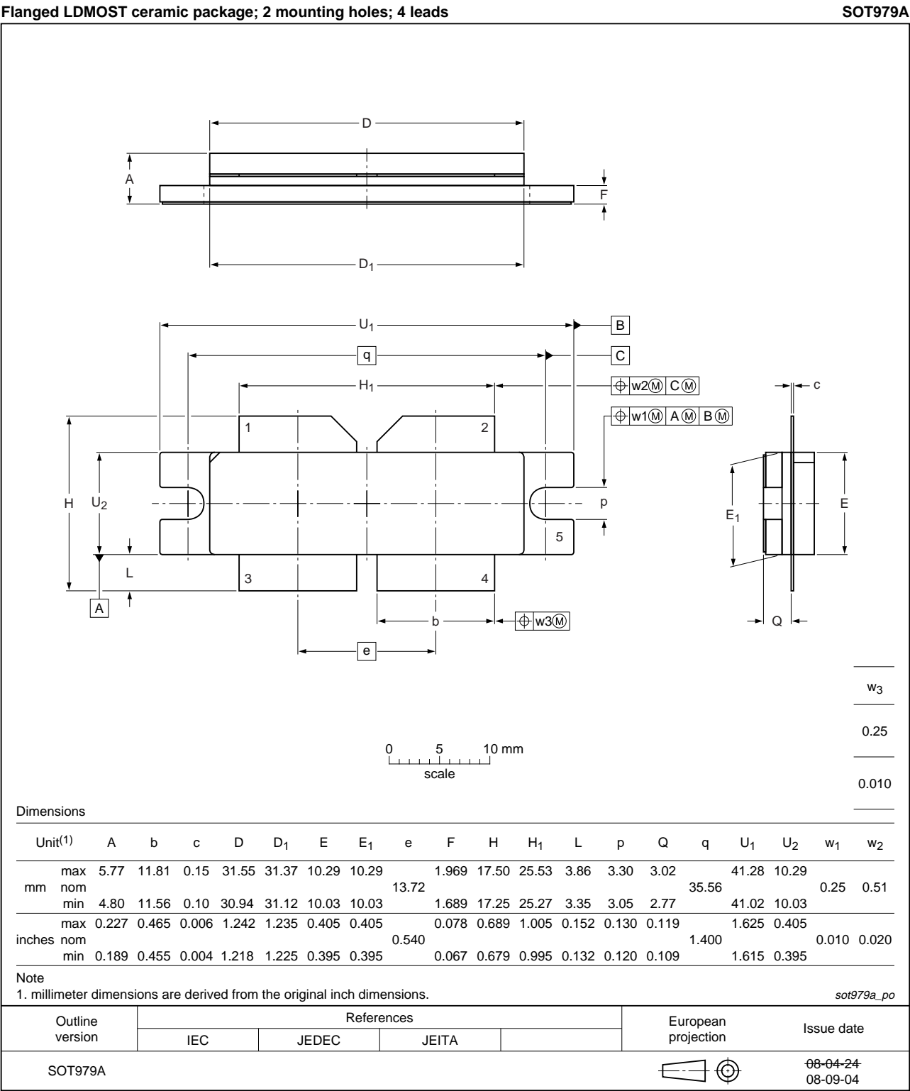
Fig 15. Package outline SOT979A
