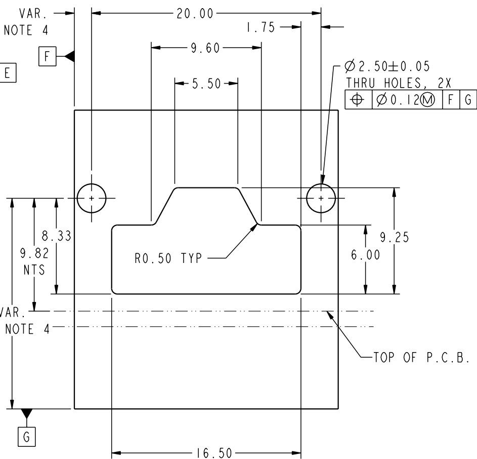
RECOMMENDED BULKHEAD OPENING
