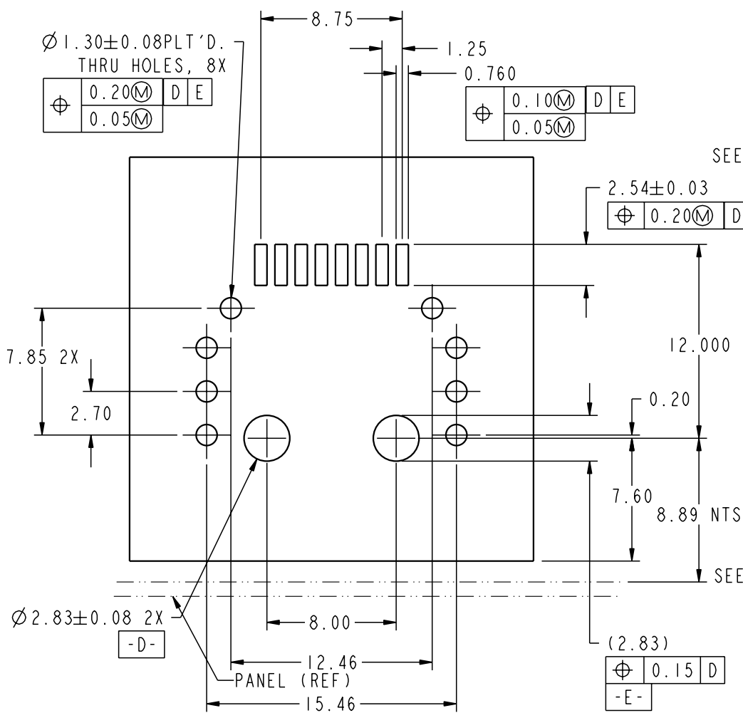
RECOMMENDED PCB FOOTPRINT AS VIEWED FROM COMPONENT SIDE
