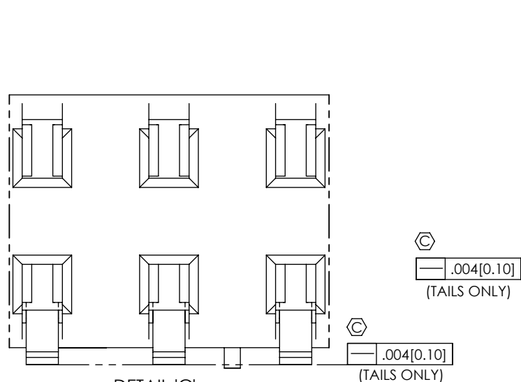
DETAIL 'C' SCALE 12:1
