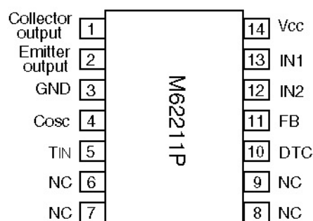
OUTLINE 14P4
