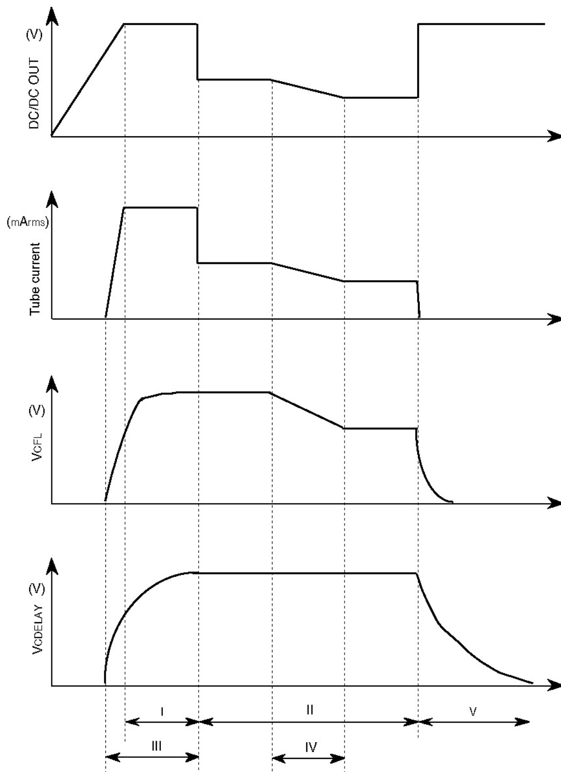
<Timing Chart>
