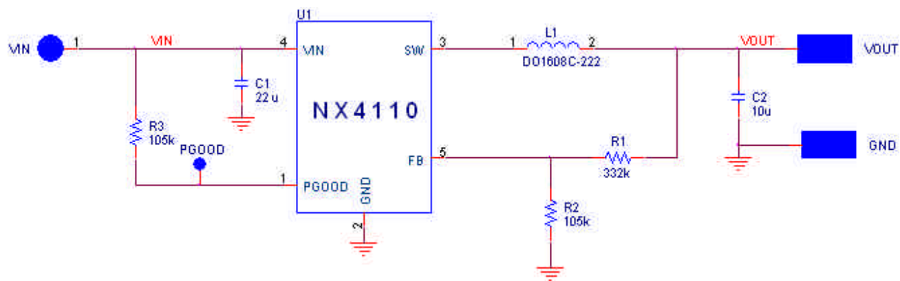
Fig. 19 - Demoboard schematic
