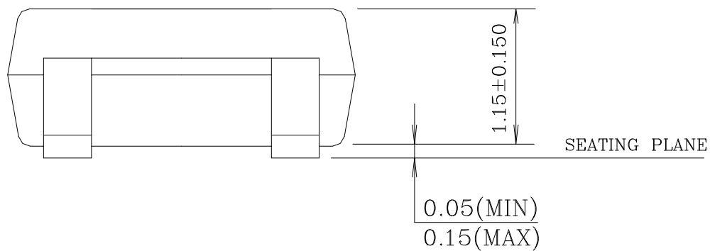
Side View
