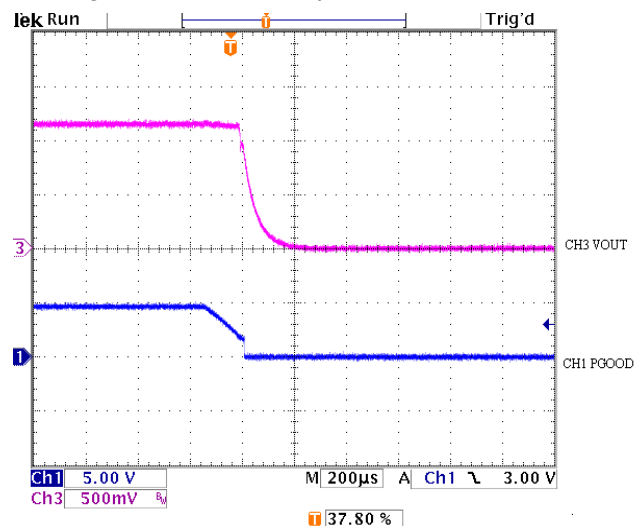
Fig. 17 - Shutdown
