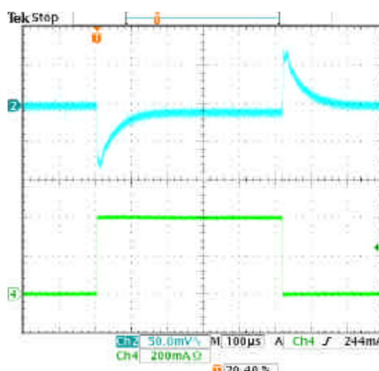
Fig. 11 - Transient response
