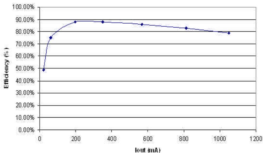
Fig. 12 - Efficiency
