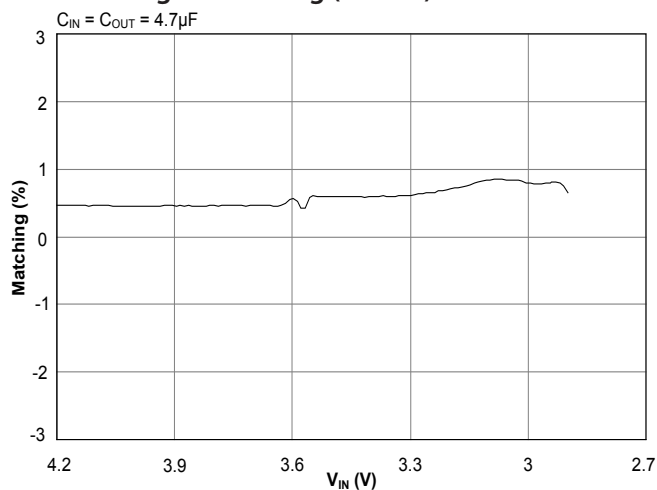
Backlight Matching (4 LEDs) — 25mA Each
