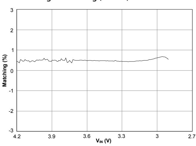
Backlight Matching (4 LEDs) — 12mA Each
