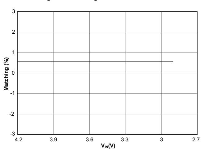
Backlight Matching (4 LEDs) — 4.5mA Each
