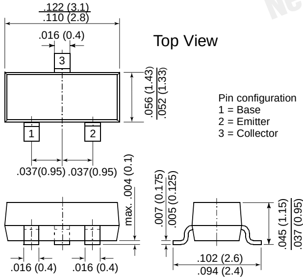
TO-236AB (SOT-23)
