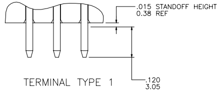
DETAIL A STANDARD PIN ONLY SCALE 10/1
