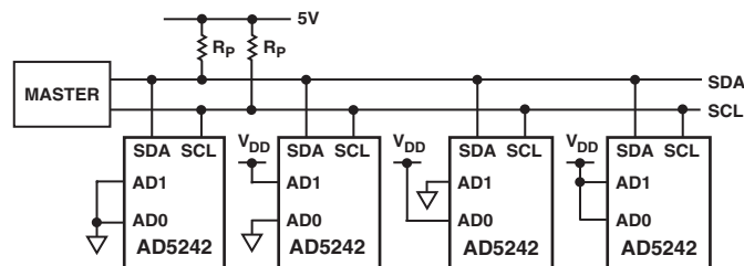
Figure 5. Multiple AD5242 Devices on One Bus
