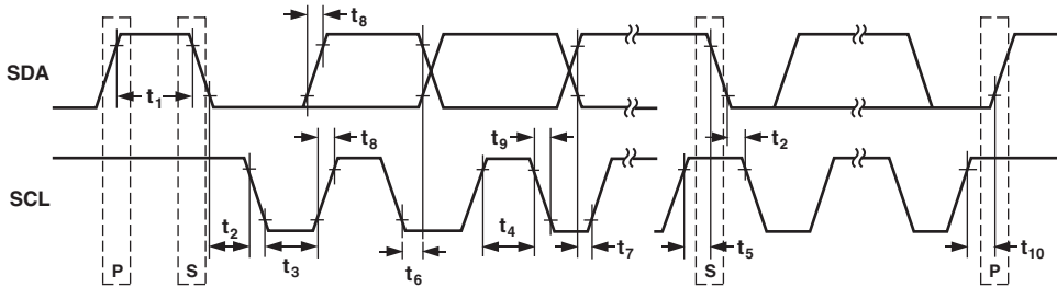
Figure 1. Detail Timing Diagram
