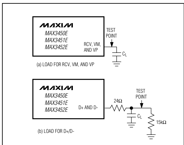
Figure 6. Test Circuits
