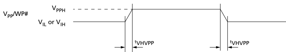
Figure 22: Accelerated Program AC Timing
