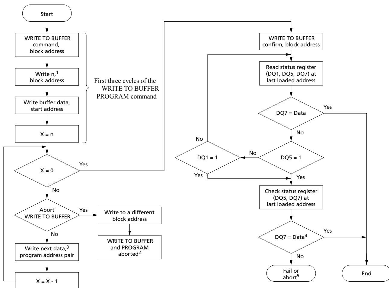
Figure 9: WRITE TO BUFFER PROGRAM Flowchart
