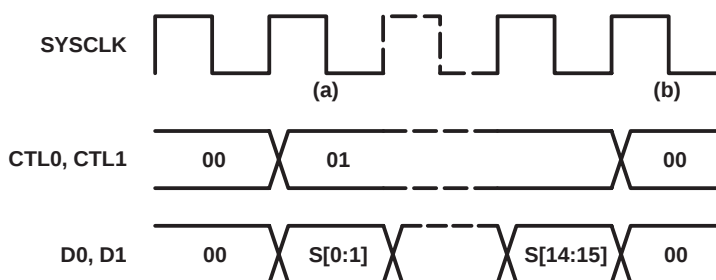
Figure 17. Status Transfer Timing
