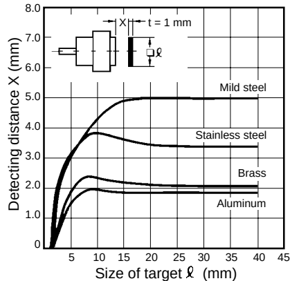
Shielded M18 sensor E2C-X5A
