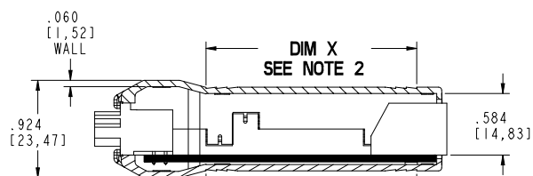
SECTION C-C
