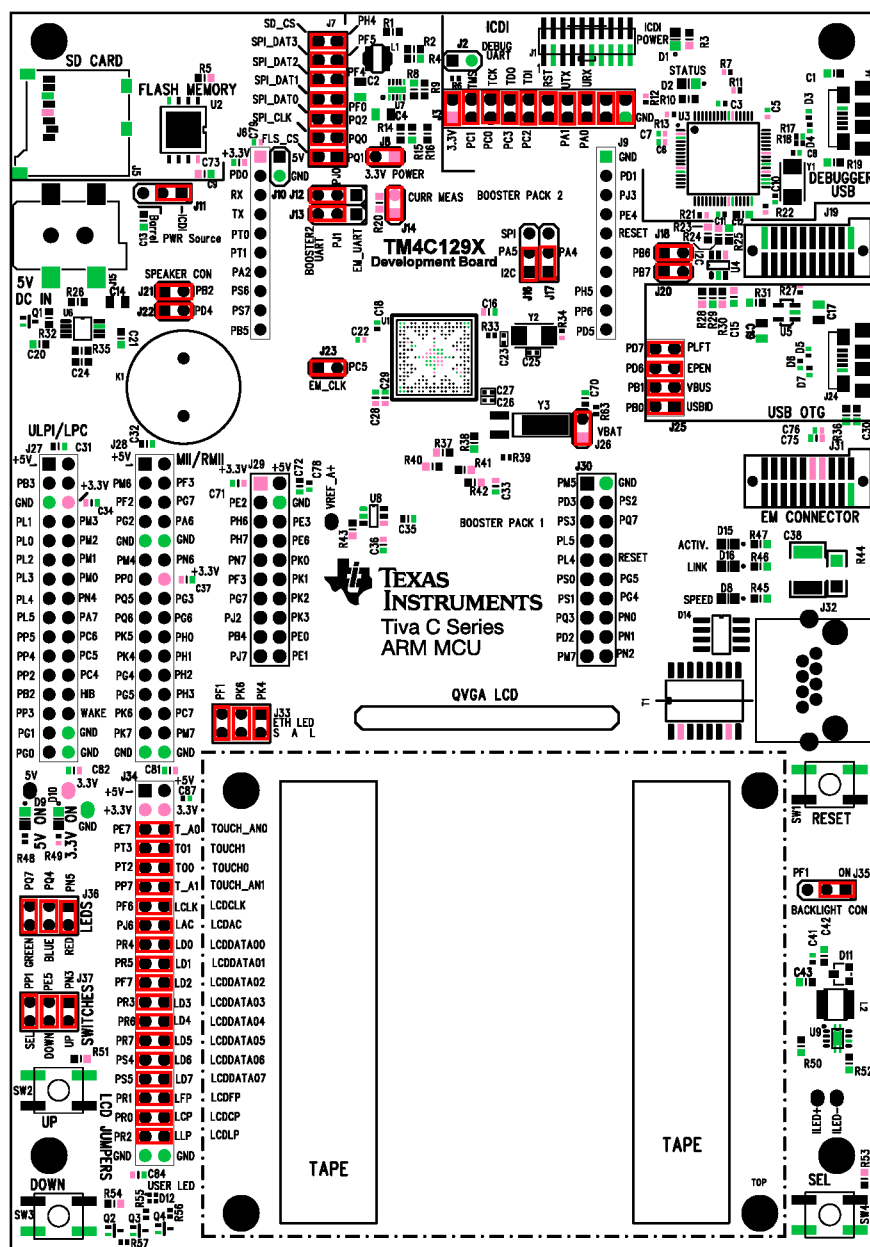
Figure A-3. Jumper sand Shunt Locations
