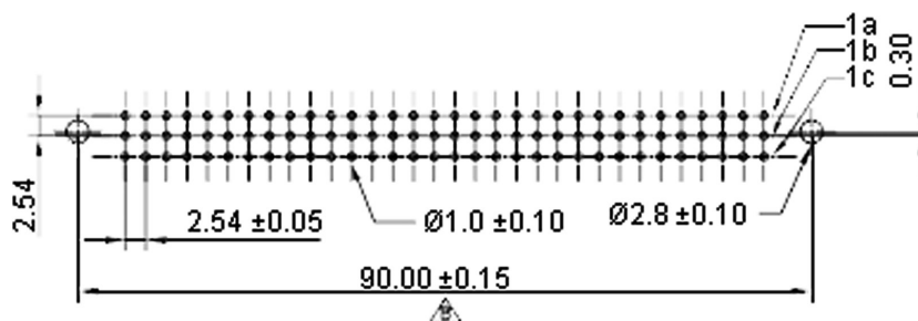
PCB Layout
