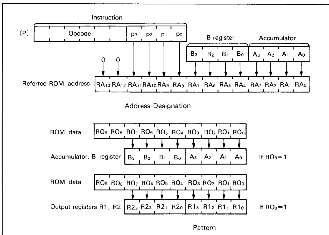
Figure 29 P Instruction
