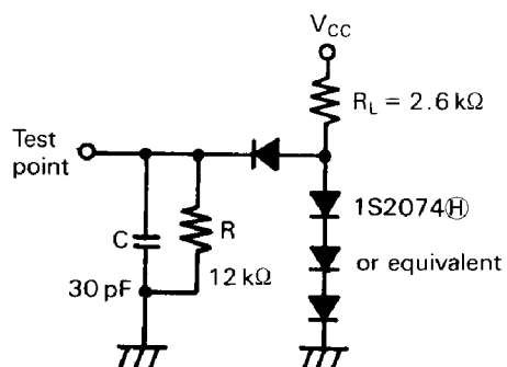
Figure 34 Timing Load Circuit
