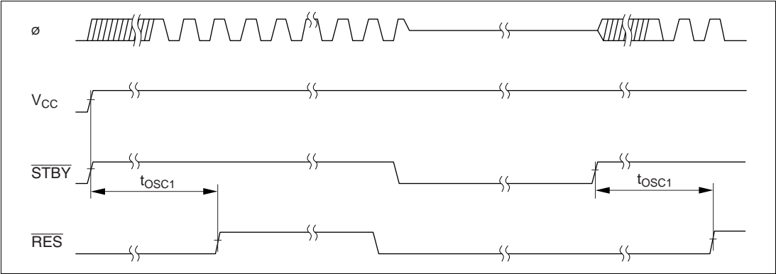
Figure 23.8 Clock Settling Timing
