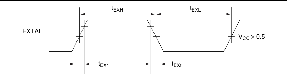
Figure 6.6 External Clock Input Timing
