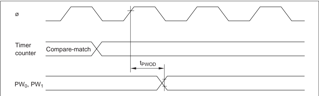
Figure 23.15 PWM Timer Output Timing
