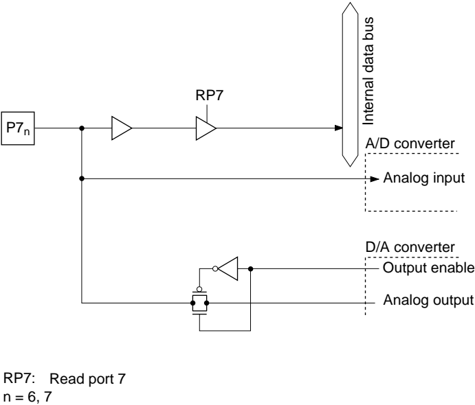
Figure C.7 (b) Port 7 Block Diagram (Pins P7 6 and P7 7 )
