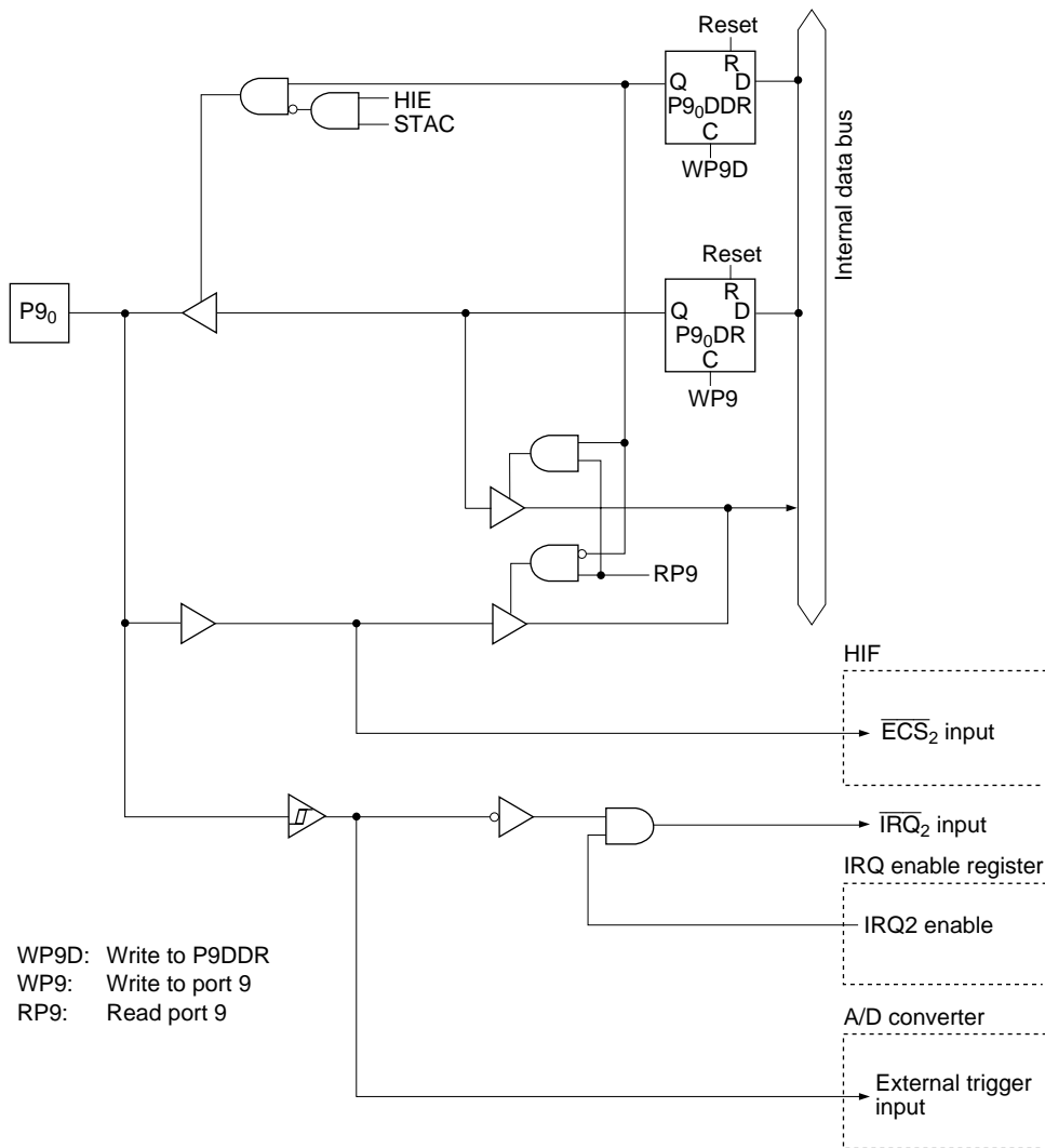
Figure C.9 (a) Port 9 Block Diagram (Pin P9 0 )
