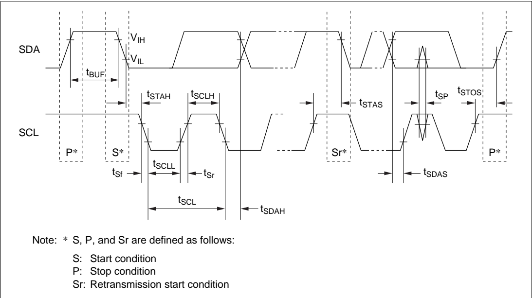
Figure 23.21 I 2 C Interface Input/Output Timing
