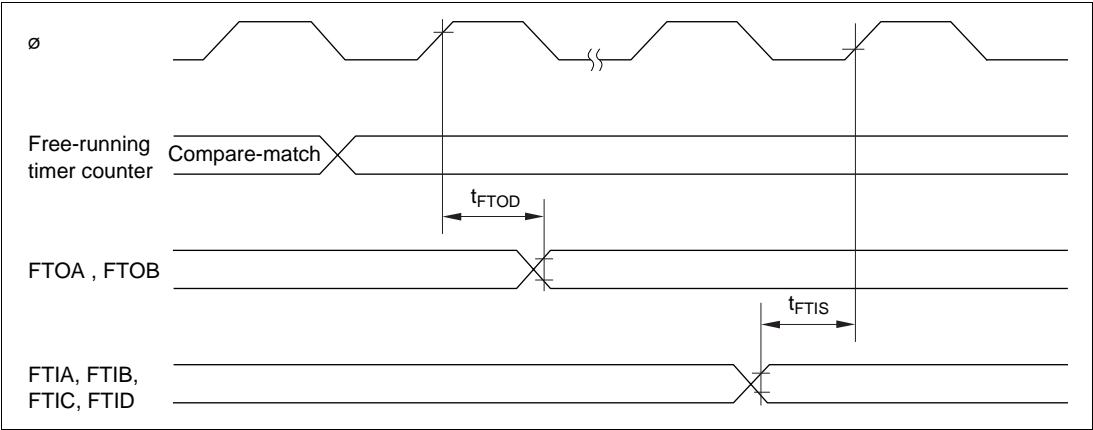
Figure 23.10 Free-Running Timer Input/Output Timing
