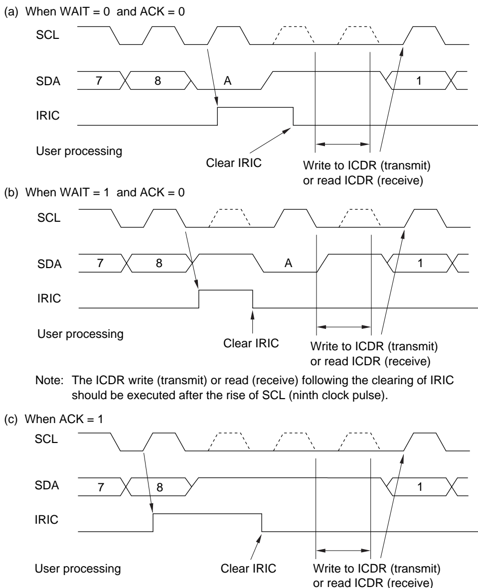
Figure 13.10 IRIC Set Timing and SCL Control
