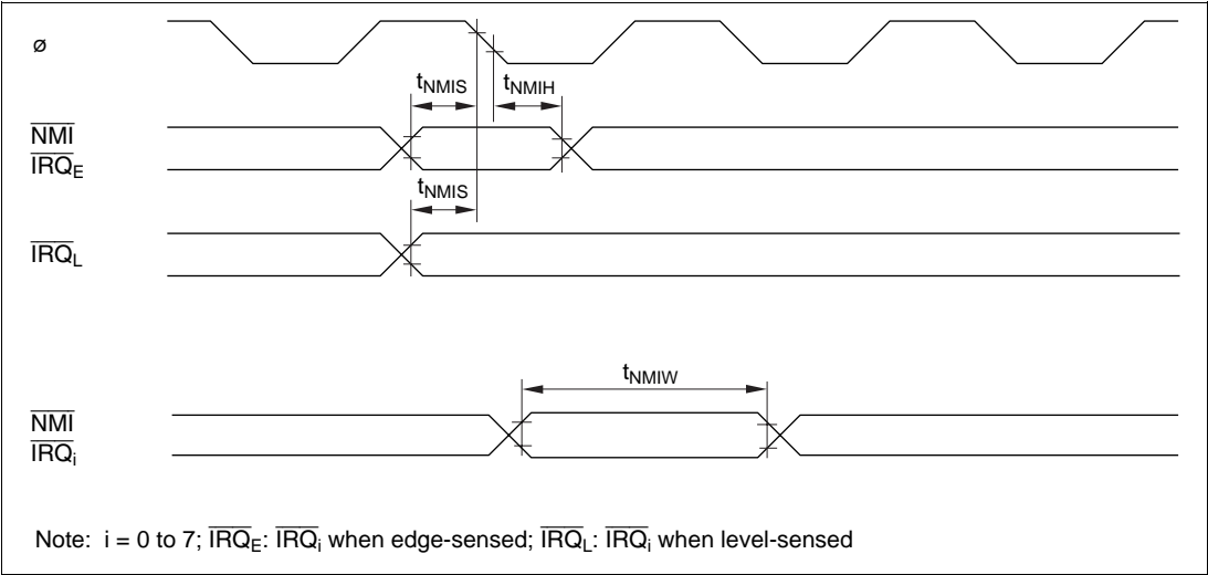
Figure 23.7 Interrupt Input Timing
