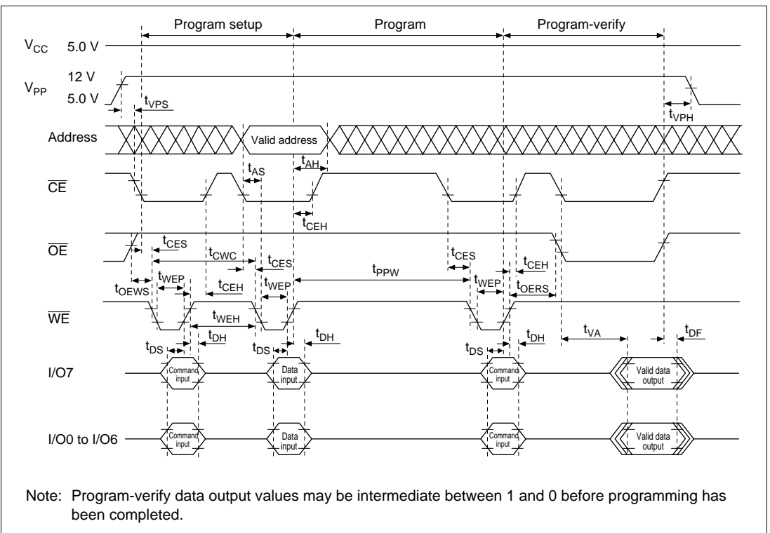
Figure 19.18 High-Speed, High-Reliability Programming Timing
