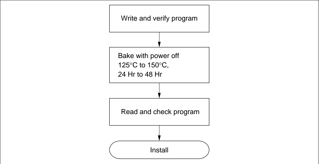
Figure 18.7 Recommended Screening Procedure
