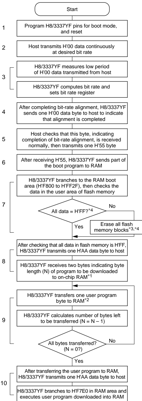
Figure 20.4 Boot Mode Flowchart
