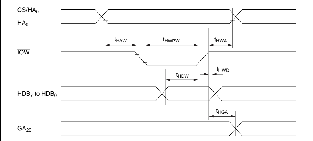
Figure 23.20 Host Interface Write Timing
