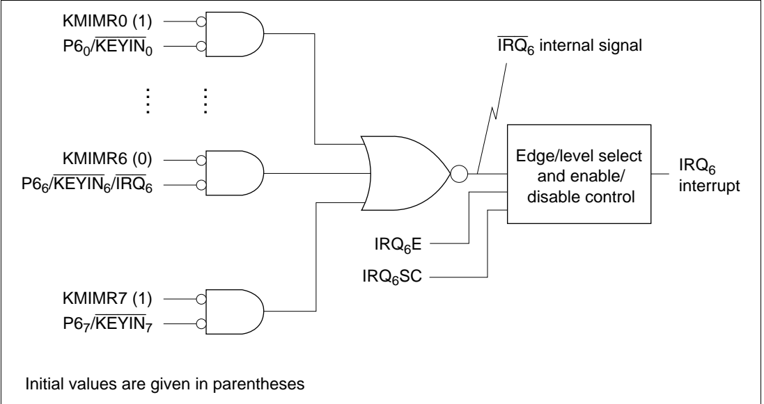
Figure 4.3 KMIMR and \text{IRQ}_6 Interrupt
