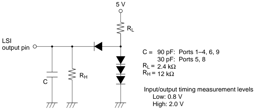
Figure 23.3 Output Load Circuit
