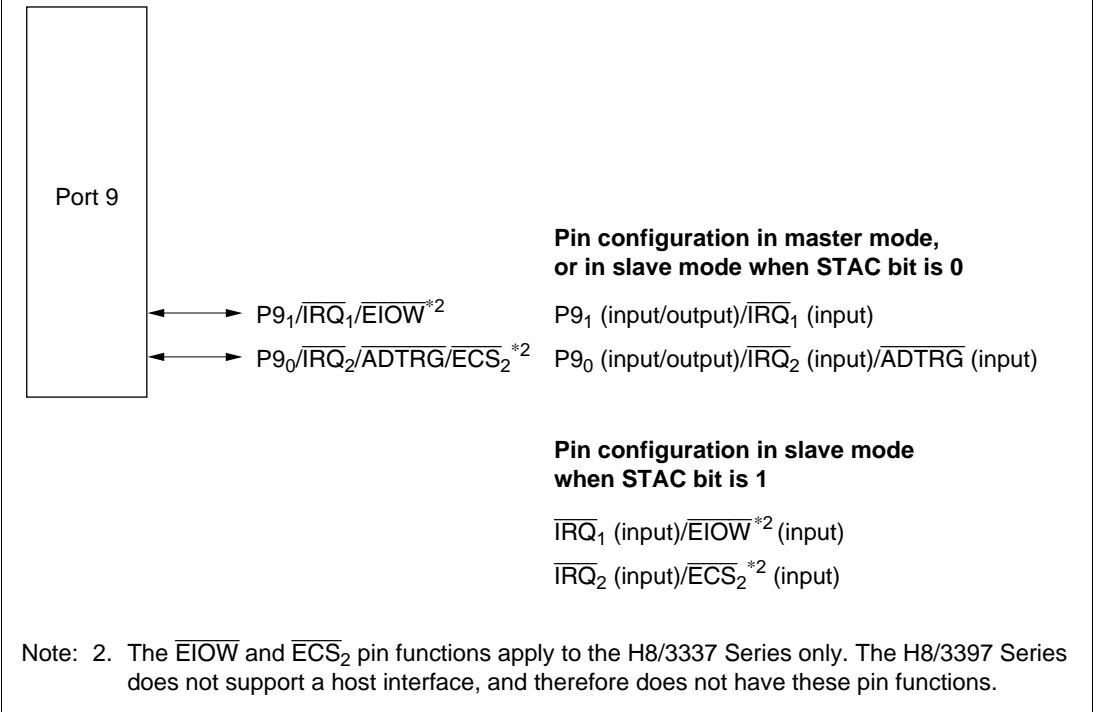
Figure 7.17 Port 9 Pin Configuration (cont)
