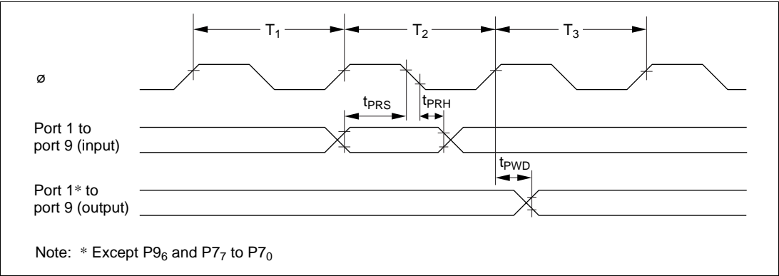
Figure 23.18 I/O Port Input/Output Timing
