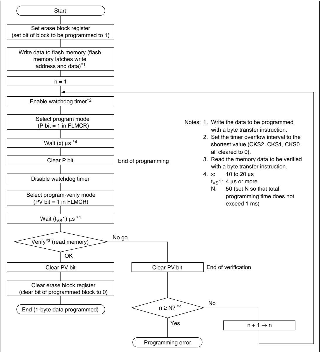
Figure 19.8 Programming Flowchart
