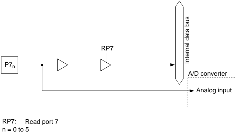
Figure C.7 (a) Port 7 Block Diagram (Pins P7 0 to P7 5 )
