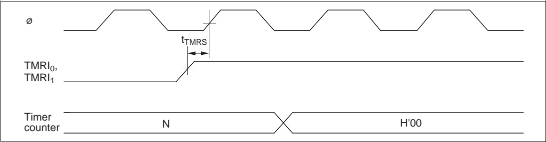
Figure 23.14 8-Bit Timer Reset Input Timing
