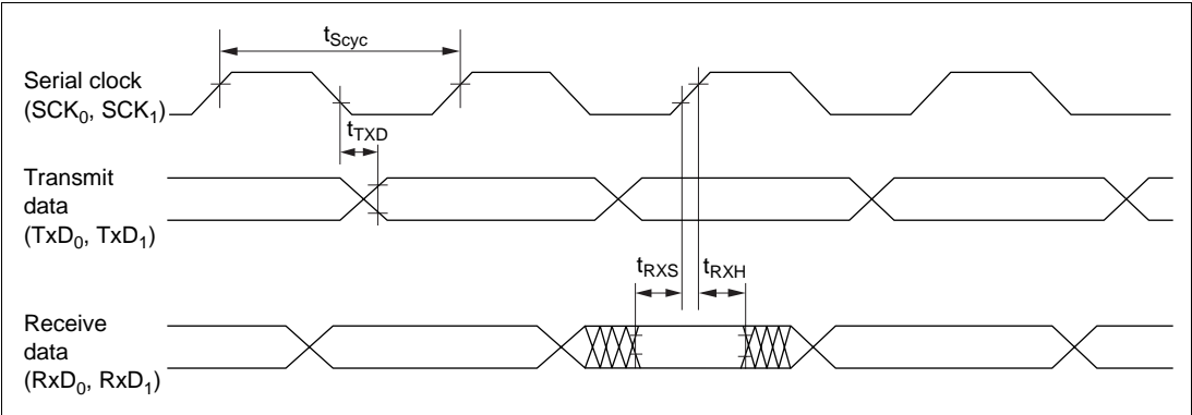
Figure 23.16 SCI Input/Output Timing (Synchronous Mode)
