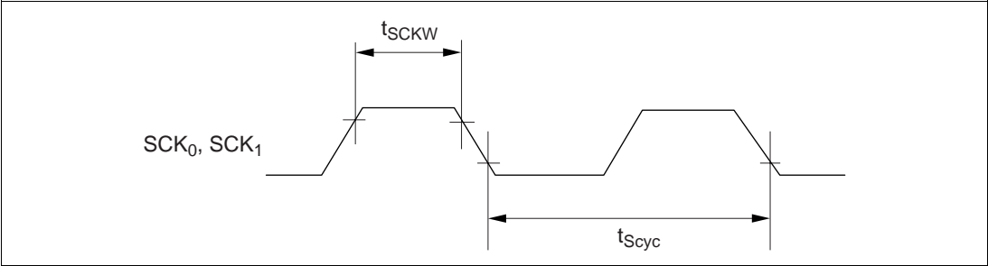
Figure 23.17 SCI Input Clock Timing
