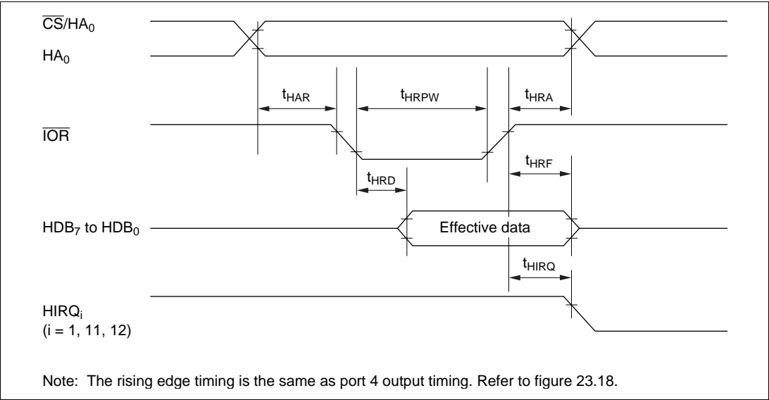
Figure 23.19 Host Interface Read Timing
