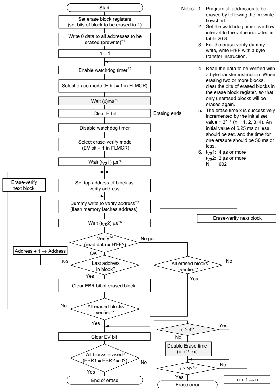
Figure 20.11 Multiple-Block Erase Flowchart
