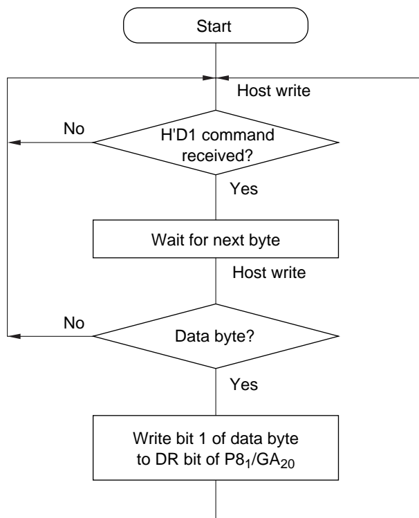
Figure 14.2 GA 20 Output
