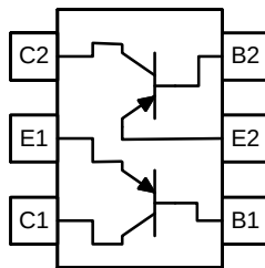
Figure 2. FMB2907A
