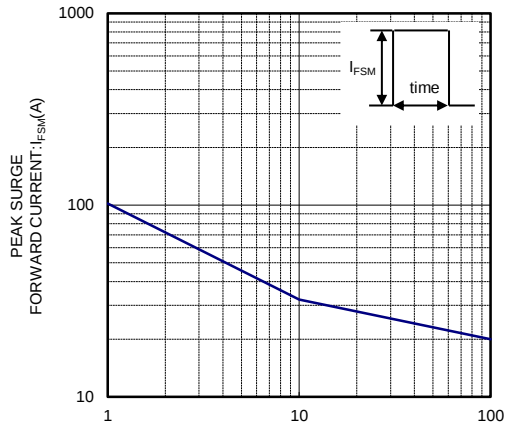
I_FSM-t CHARACTERISTICS
