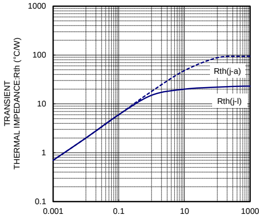
R_th-t CHARACTERISTICS
