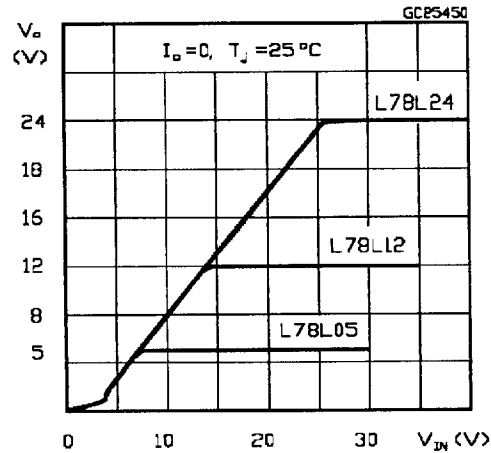
Figure 6: L78L05/12/24 Output Characteristics.
