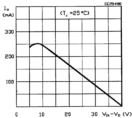
Figure 9 : L78L00 Series Short Circuit Output Current.
