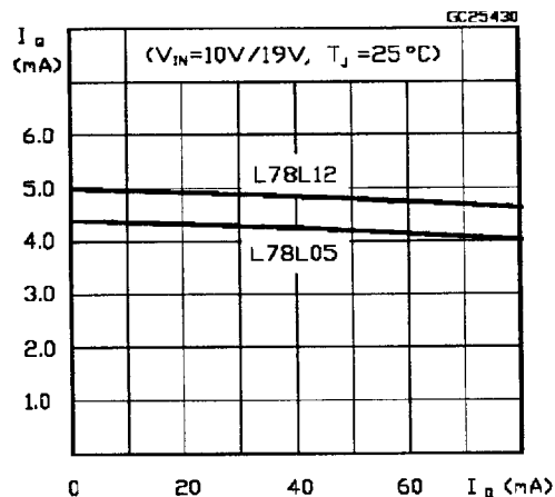
Figure 4: L78L05/12 Quiescent Current vs Output Current
