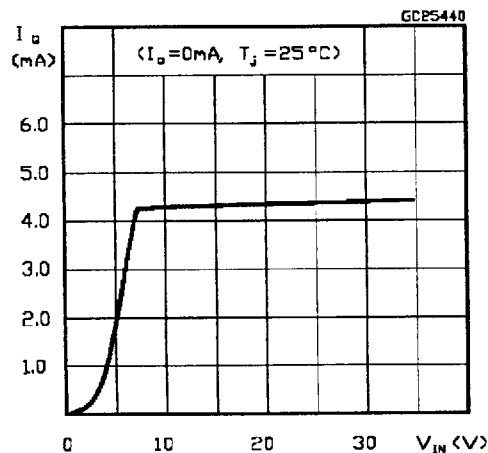
Figure 5: L78L05 Quiescent Current vs Input Voltage.
