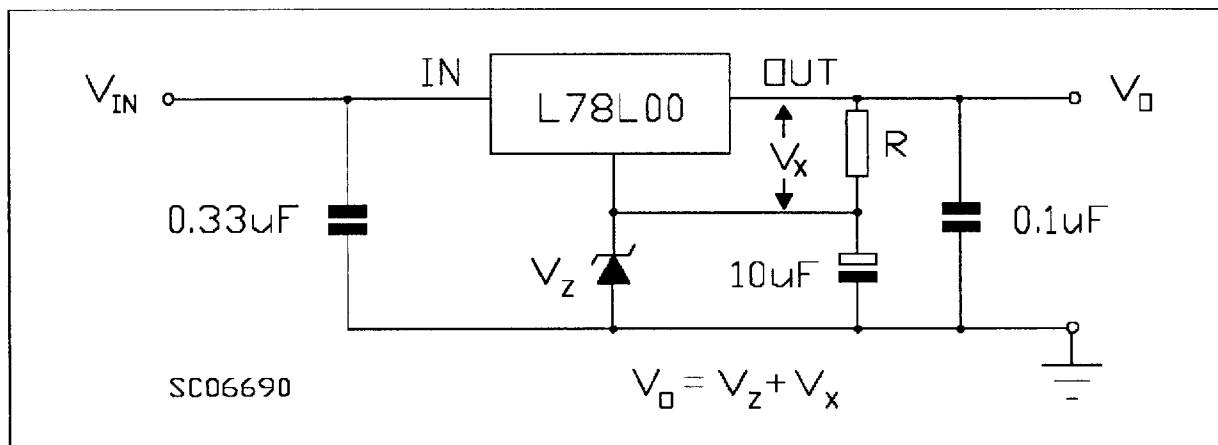
Figure 12 : Current Regulator.
