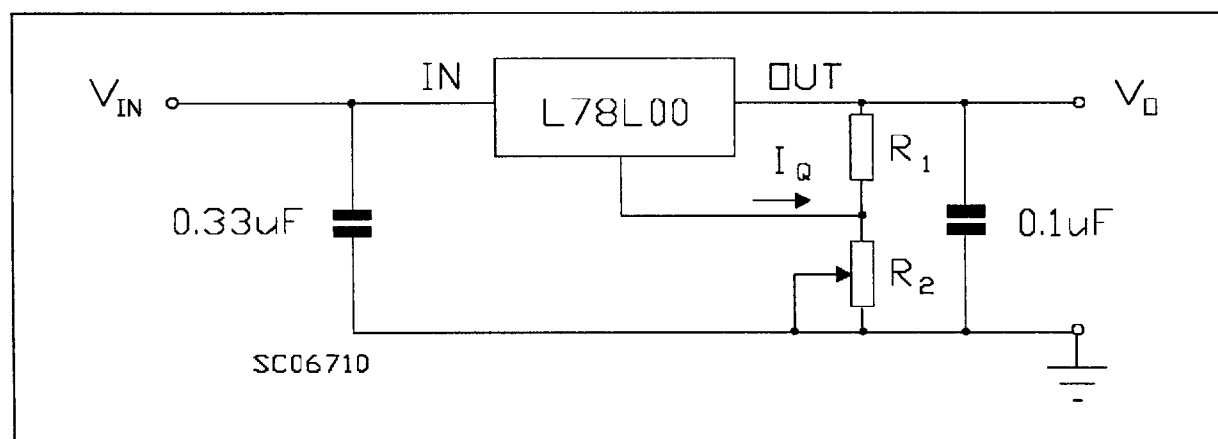
Figure 13: Adjustable Output Regulator
