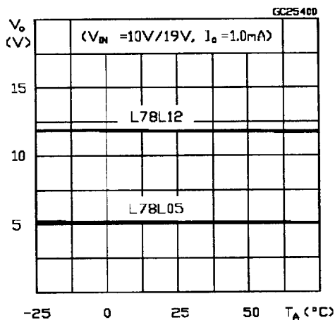
Figure 1: L78L05/12 Output Voltage vs Ambient Temperature
