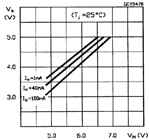
Figure 8 : L78L05 Dropout Characteristics.
