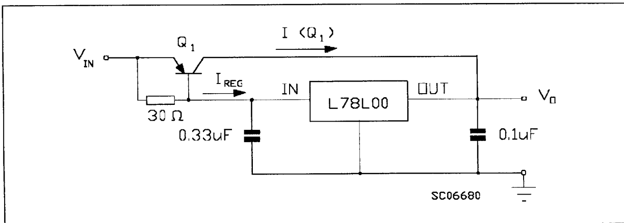
Figure 10: High Output Current Short Circuit Protected
