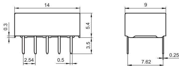
Outline Dimensions
