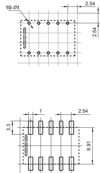
PCB Layout (Bottom view)
