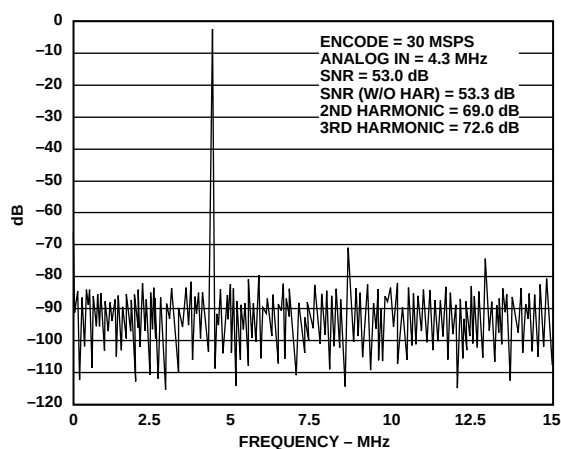
Figure 11. FFT Plot 30 MSPS, 4.3 MHz
