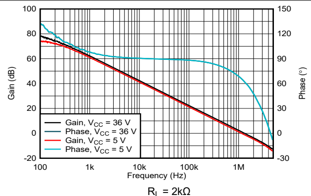
Figure 5-6. Open-Loop Gain and Phase vs Frequency
