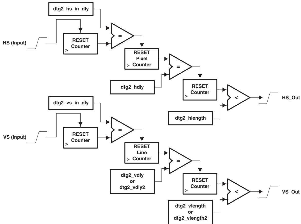
Figure 4-15. THS8200 DTG VS/HS Output Generation
