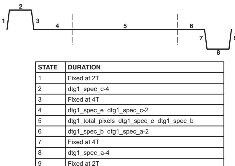
Figure 4-19. HDTV Line Type FULL_NTSP
