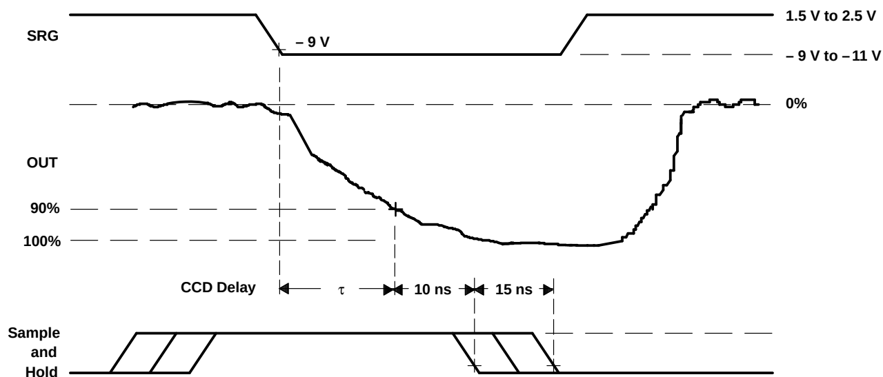
Figure 13. SRG and CCD Output Waveforms
